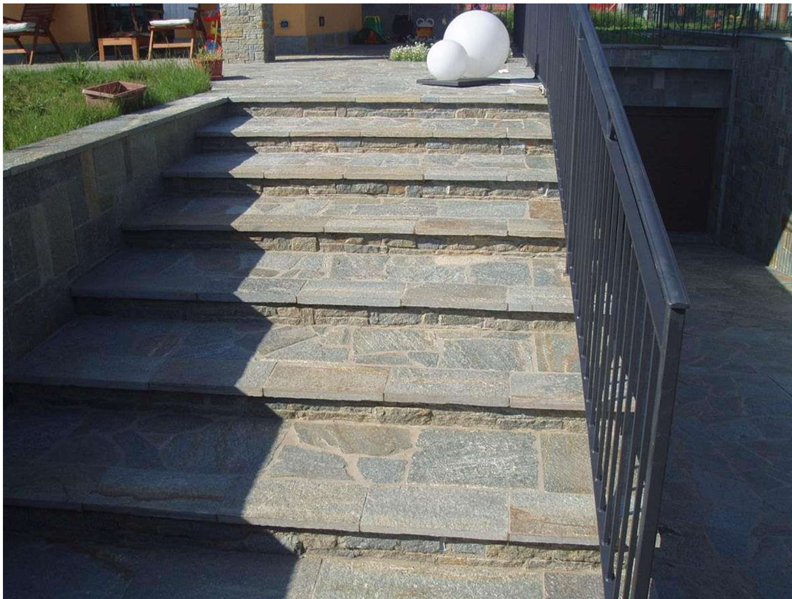
gradoni-in-lastre-di-Luserna 1
